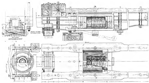
Figs. 3943-3946. Hinson Friction Draft Gear. National Car Coupler Co.
